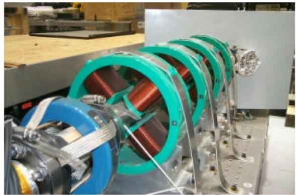
Figure 3 : MIRFEL Quadrupole magnets
