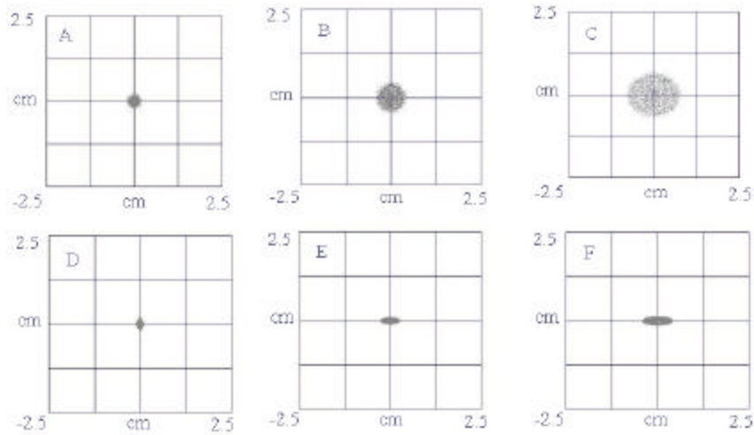
Figure 5 : xy plots at various points along the beamline. (A) At the photocathode (B) Exit of RF gun (C) Exit of booster section (D) Upstream cavity mirror aperture (E) Wiggler center (F) Wiggler Exit
