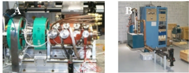
Figure 1 : (A) RF Gun (B) 2856 MHz Klystron
