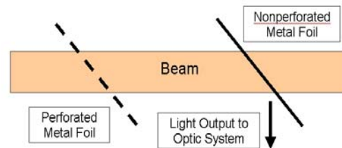
Figure 1: ODR-OTR interferometer; interferences between forward directed ODR from a mesh inclined at 45^\circ and backward reflected OTR from a parallel mirror are observed at 90^\circ with respect to the beam direction.
