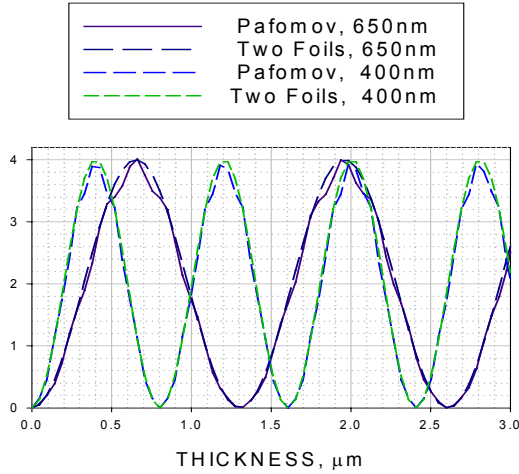
Figure 4: The Pafomov and two metal foil model of dielectric foil radiation for two different wavelengths.
