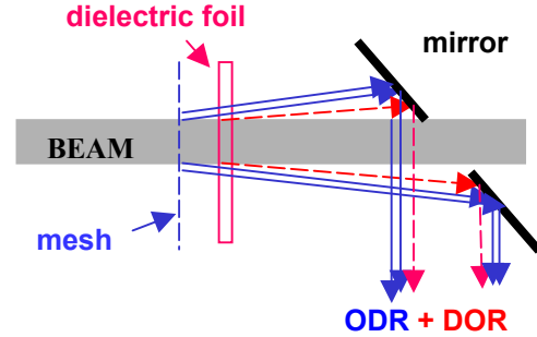
Figure 3: Mesh-dielectric foil interferometer.
