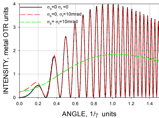
Figure 5: Effect of beam divergence on OTR-DOR interferences.
