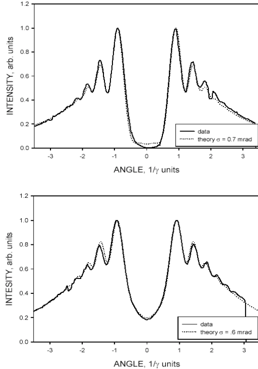
Figure 2: (top): fit of a vertical scan of OTR-OTR interference pattern to computer generated simulation; (bottom): similar fit to vertical scan of ODR-OTR interference pattern with theoretical calculation.
